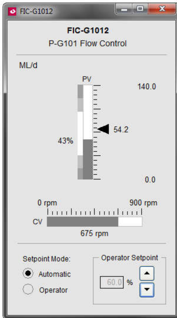
Figure 2-9: Sample PID Controller Equipment Faceplate
