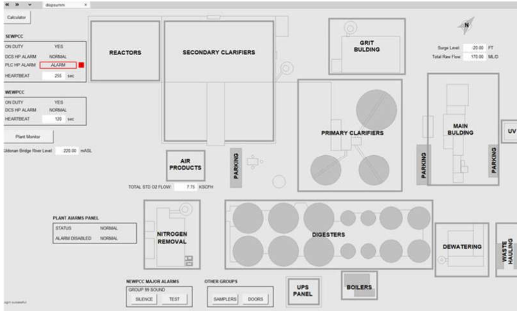
Figure 2-2: Sample Overview Navigation Display
