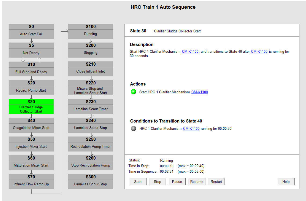
Figure 2-6: Sample Process Detail Display for a Sequencer
